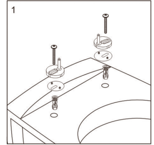
1 Insert the hinges into the toilet.
