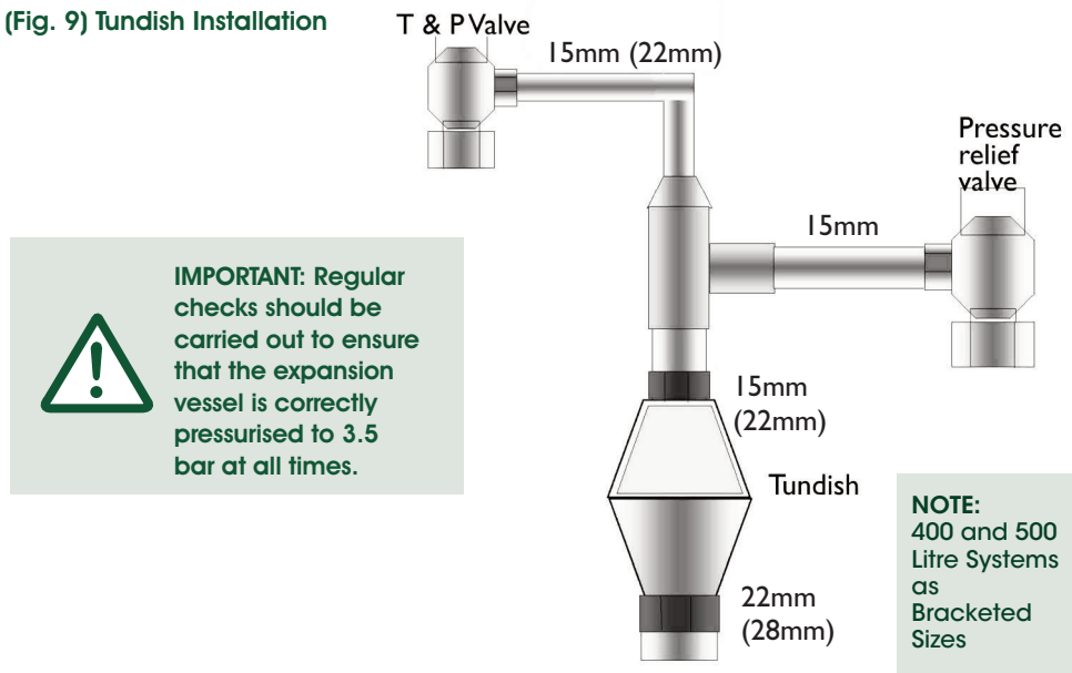
(Fig. 9) Tundish Installation
