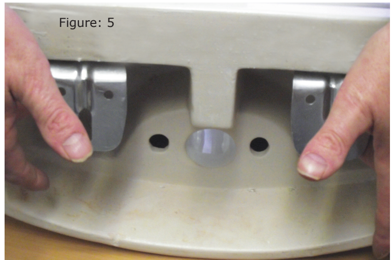
Figure 5: Fasten wall brackets to cavity wall firmly using silicone sealant along rear of basin for extra strength. Slide basin over wall brackets. Run bead of silicone around rear of basin to finish.
