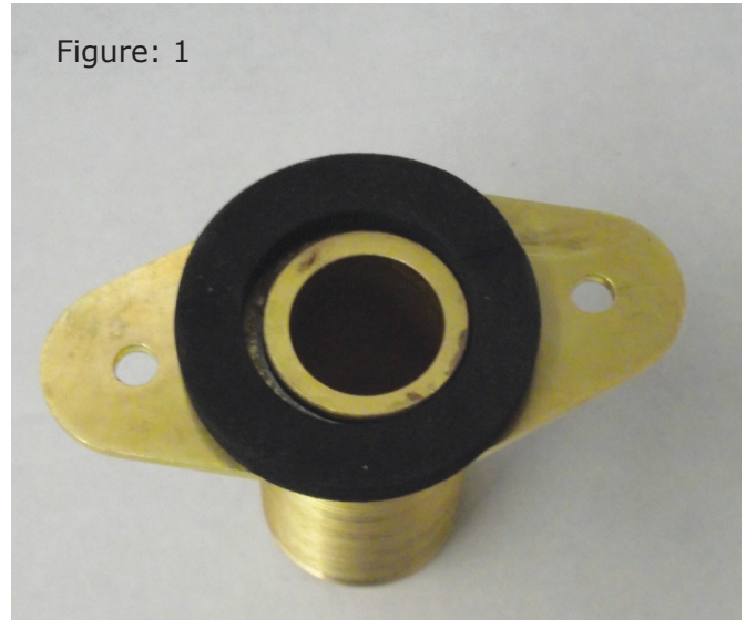
Figure: 1 Put seal on the end of waste fixing and place over waste outlet at rear of basin. See Figure 2.
