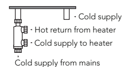
Connections for Packs J, M, P, Q, R and S
