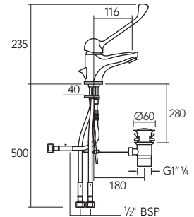
Streamline 2000 elbow lever
