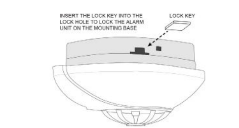
FIGURE 7 – LOCKING THE ALARM UNIT WITH THE BASE
