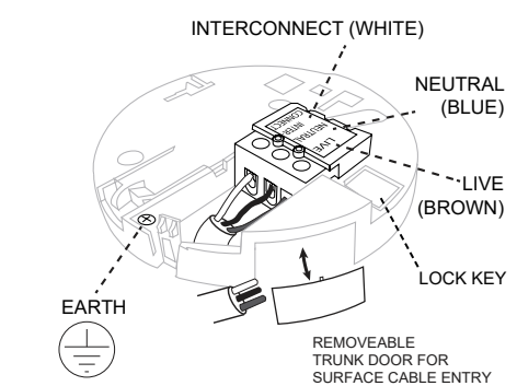
FIGURE 5 – WIRING & INTERCONNECT FACILITY
