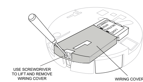
FIGURE 6 – REMOVE WIRING COVER
