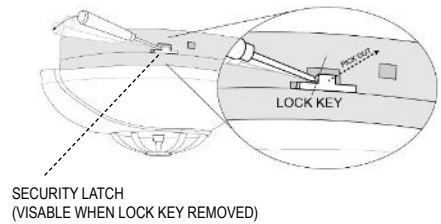
FIGURE 8 – USE SCREW TO PICK OUT THE LOCK KEY FROM THE MOUNTING BASE
