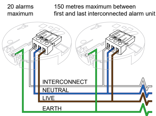
FIGURE 4 – WIRING AND INTERCONNECT
