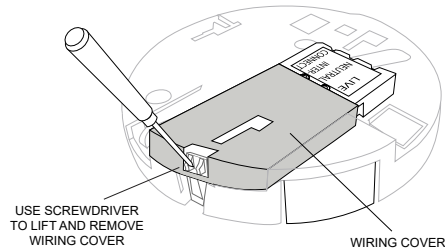
FIGURE 6 – REMOVE WIRING COVER
