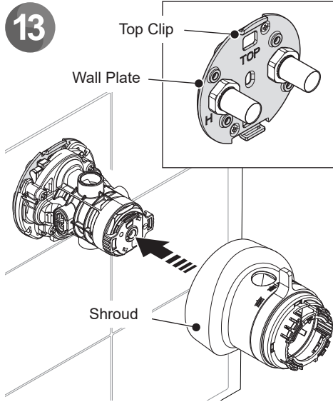
Mixing Valve
