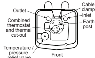
Figure 7 – 3kW model
