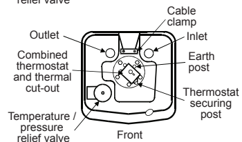
Figure 7 – 4.5kW model
