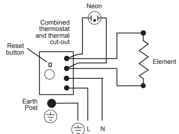
Figure 3 – 4.5kW model
