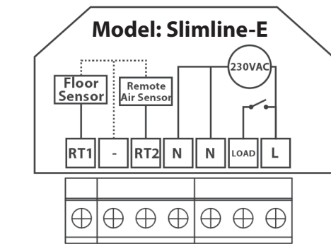
Wiring Detail
