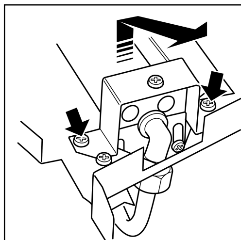
Figure 32. Removal of burner
