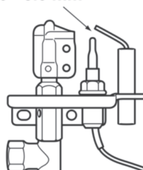
Figure 6. Pilot spark gap Note: Pilot style may vary)
