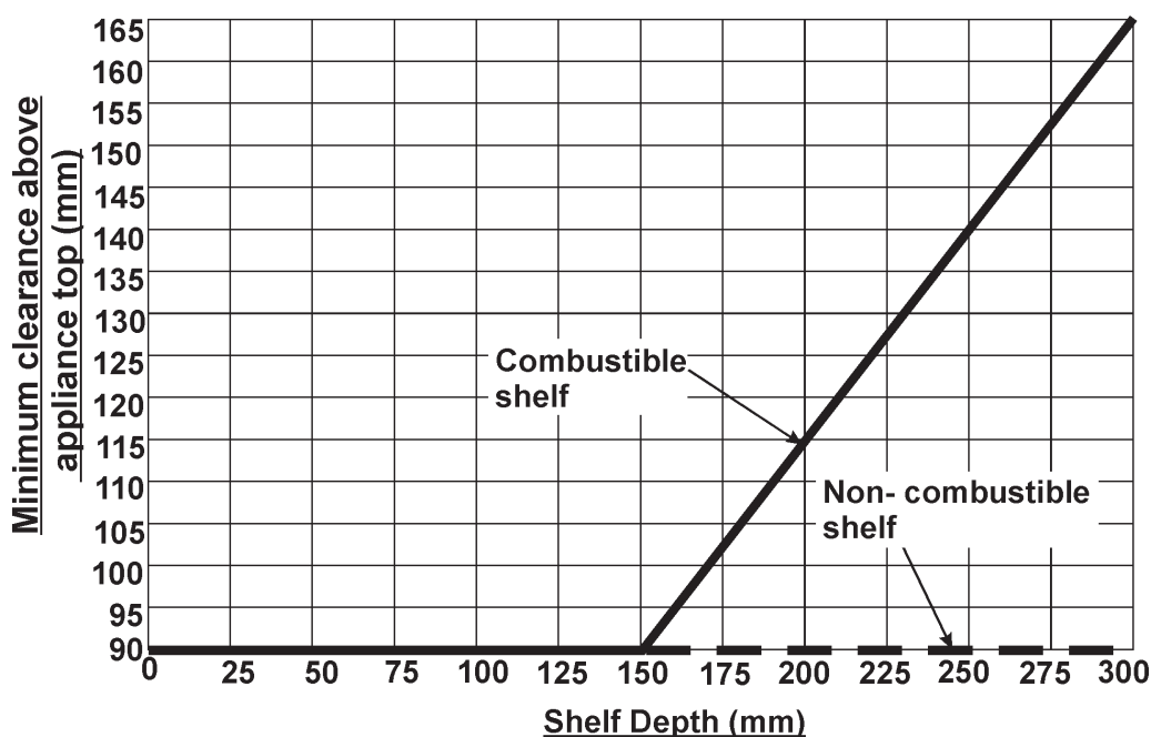
Figure 1. Shelf clearances
