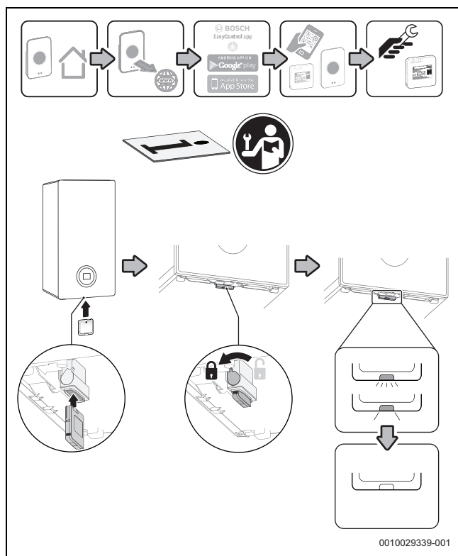
Fig. 6 Installing Key
