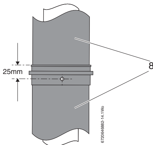
Fig. 25 Flue connection
