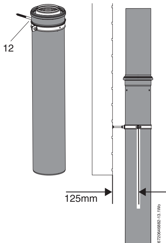
Fig. 23 Flue support
