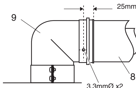
Fig. 15 Securing the extension
