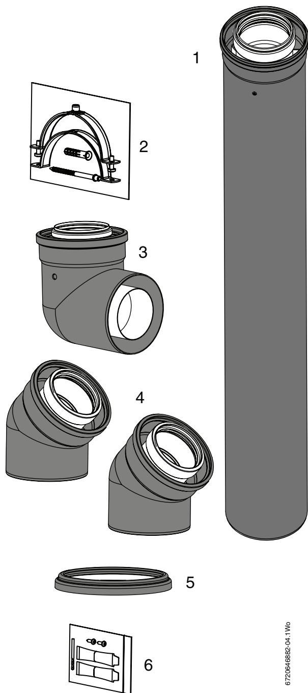
Fig. 4 Extension components
