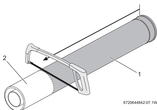
Fig. 10 Shortening a flue extension
