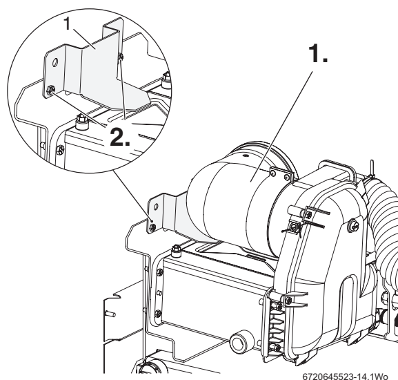
Fig. 20 Securing bracket
